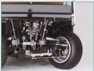
Automotive type Double-wishbone Front suspension
